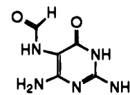
guanine-Fapy
