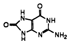
7,8-dihydro-8-oxoguanine
